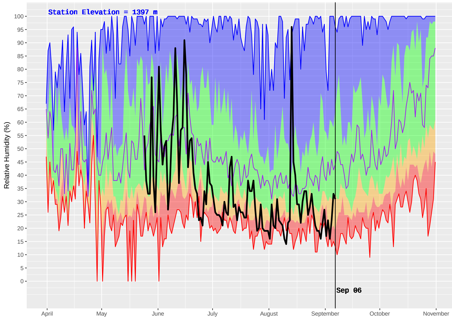
NANCY GREEN (407) : Historical (1992–2016) and Current (2017) Noon Relative Humidity
