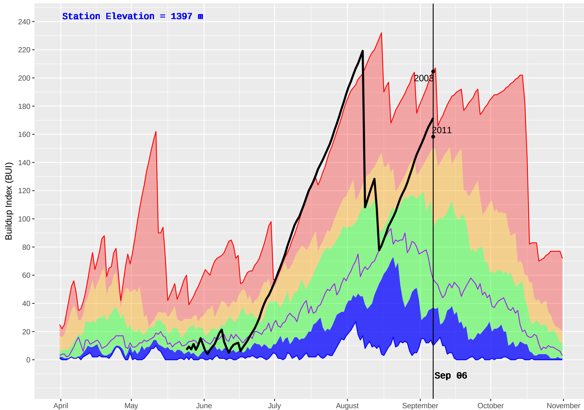
NANCY GREEN (407) : Historical (1992–2016) and Current (2017) Noon Buildup Index (BUI)
